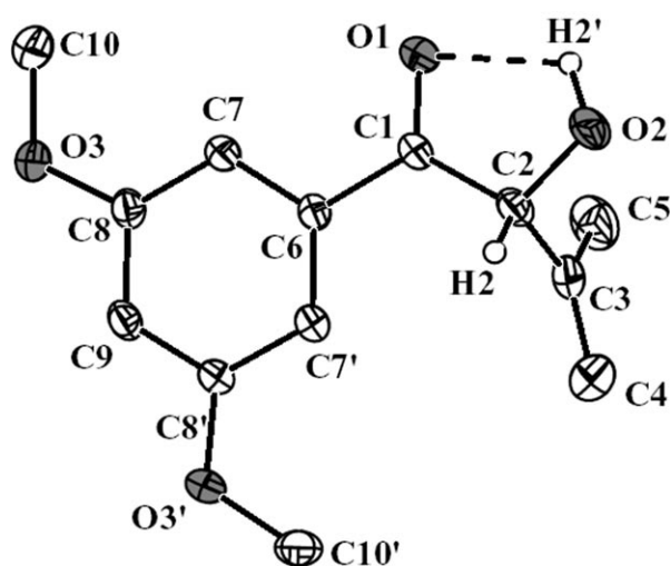
Figure 1. Molecular structure of 20e showing the conformation.
