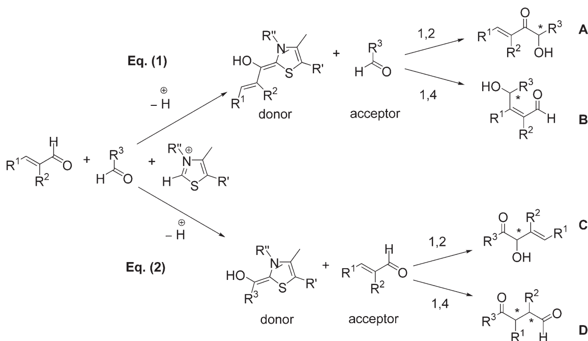
Scheme 1. ThDP-dependent catalytic reaction possibilities of \alpha,\beta -unsaturated aldehydes.
