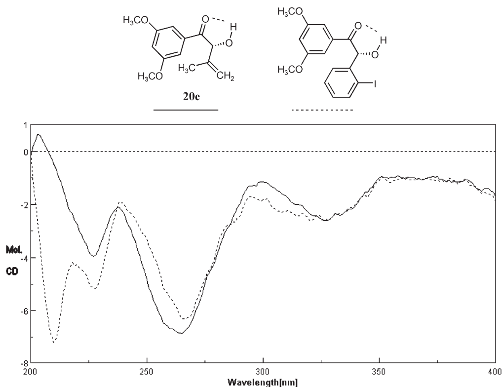
Figure 2. CD spectra of ( R )-1-(3,5-dimethoxyphenyl)-2-hydroxy-3-methylbut-3-en-1-one ( 20e , solid line) in comparison to ( R )-2-(2-iodophenyl)-1-(3,5-dimethoxyphenyl)-2-hydroxyethanone [8] (dashed line).
