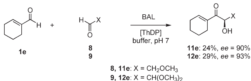
Scheme 2. Reaction of cyclohex-1-enecarbaldehyde ( 1e ) and the acetaldehyde derivatives 8 and 9 catalysed by BAL.
