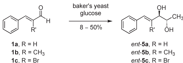
Scheme 3. Baker's yeast-catalysed transformation of \alpha,\beta -unsaturated aldehydes. [36,37]
